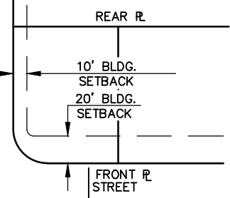
TYPICAL CORNER LOT BUILDING SETBACKS
